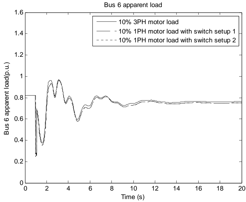
Figure 6-11 Bus 6 load apparent power for 10% motor load
