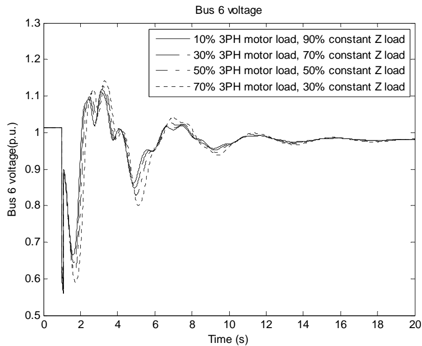
Figure 6-3 Bus 6 voltage magnitude for three-phase motor load
