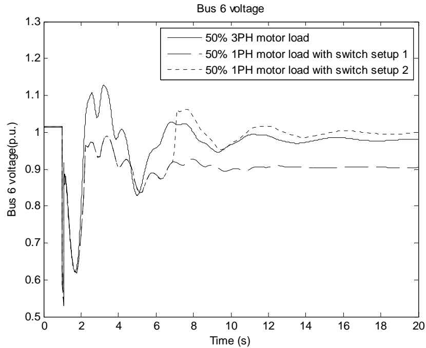
Figure 6-16 Bus 6 voltage magnitude for 50% motor load
