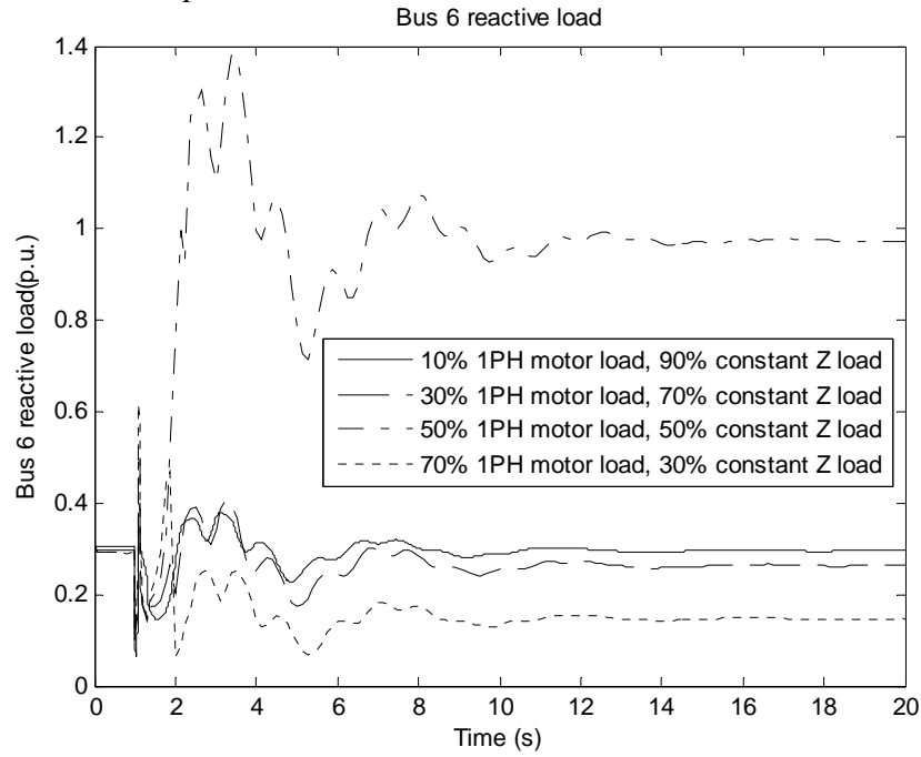
(b) Bus 6 load reactive power
