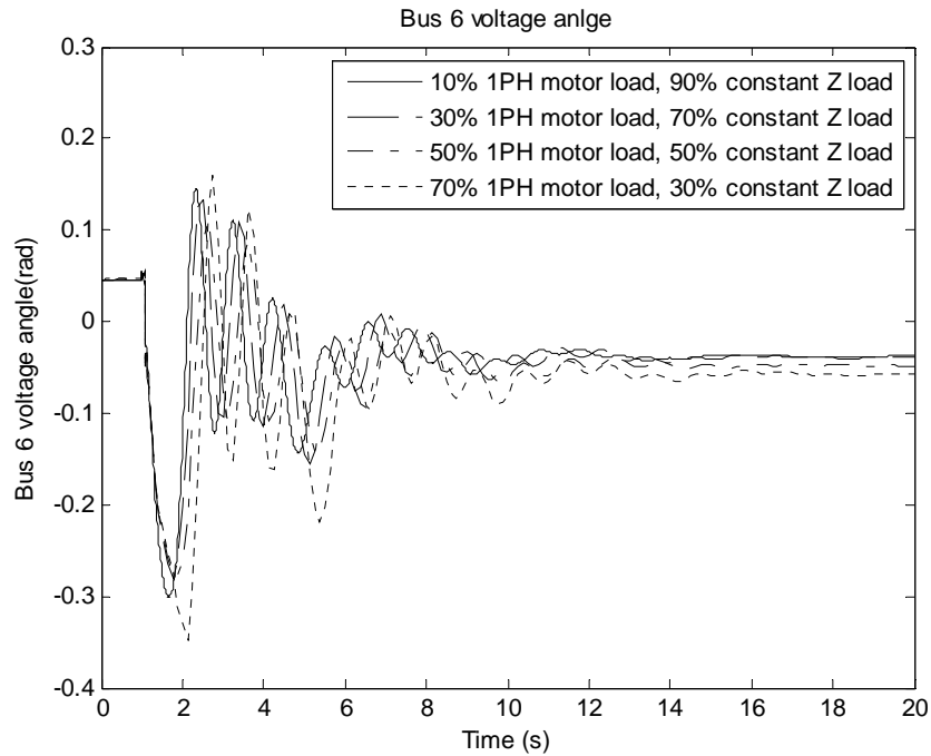
Figure 6-7 Bus 6 voltage angle with protection setup 1
