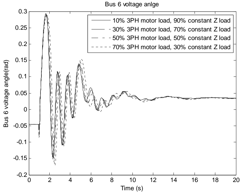
Figure 6-4 Bus 6 voltage angle for three-phase motor load
