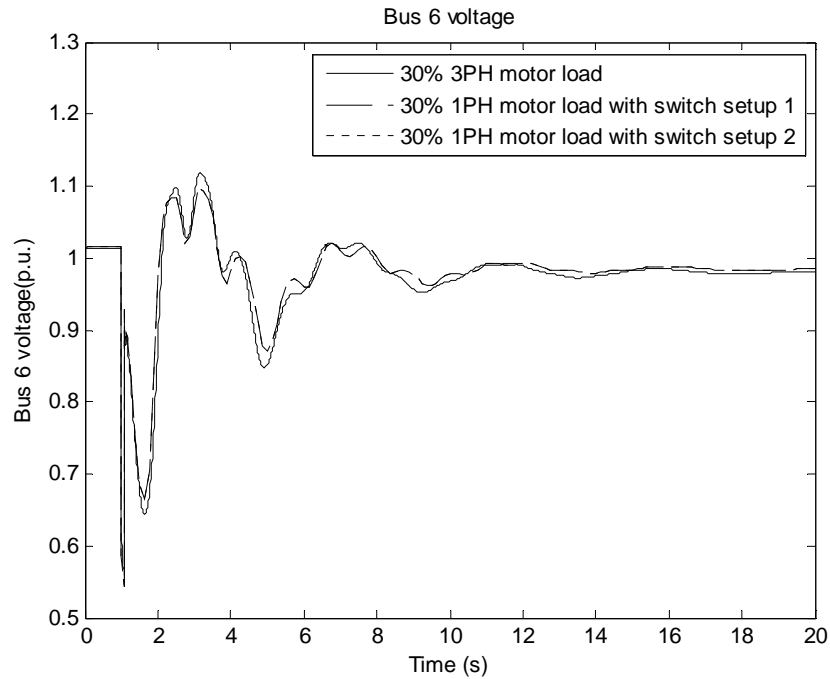
Figure 6-14 Bus 6 voltage magnitude for 30% motor load
