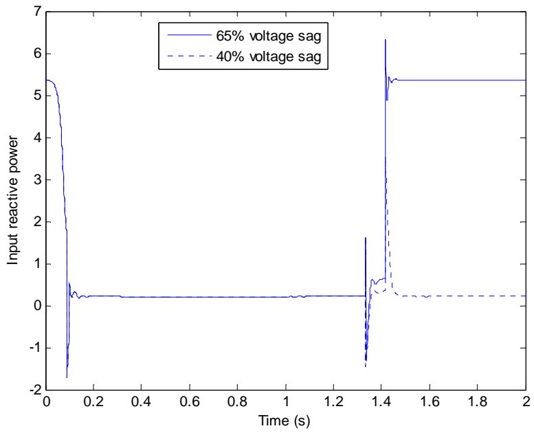
(c) The input reactive power (p.u.)
