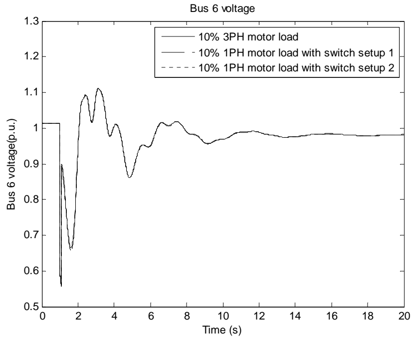
Figure 6-12 Bus 6 voltage magnitude for 10% motor load
