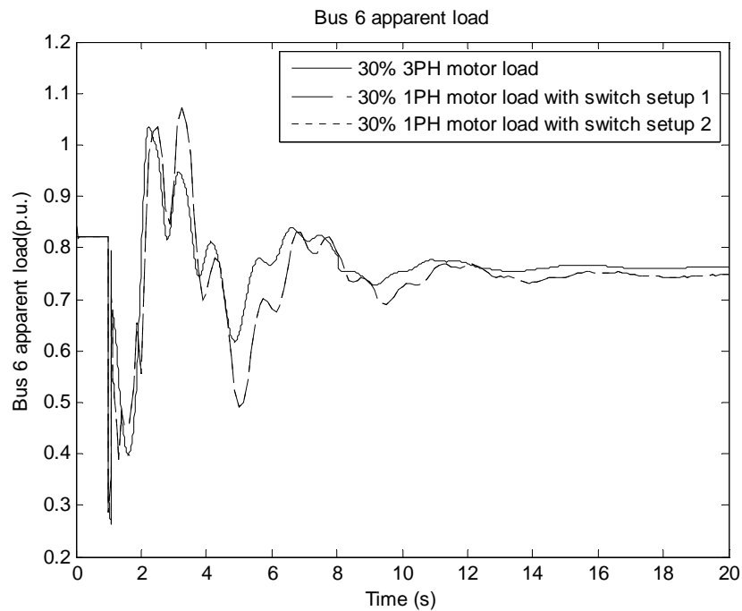
Figure 6-13 Bus 6 load for 30% motor load
