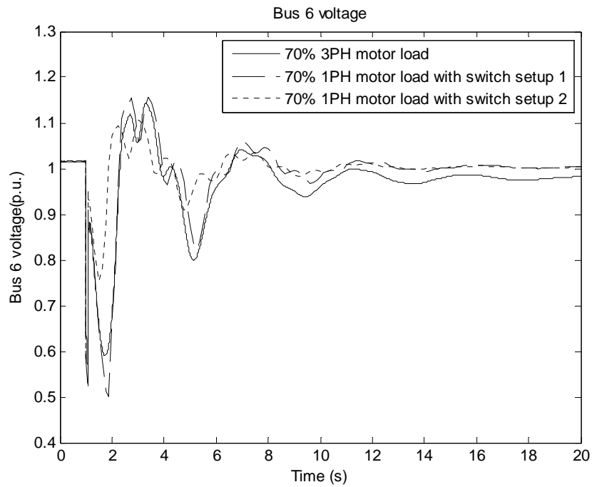
Figure 6-18 Bus 6 voltage magnitude for 70% motor load
