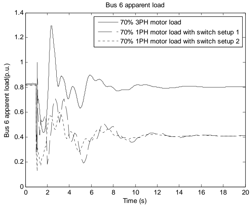
Figure 6-17 Bus 6 load for 70% motor load
