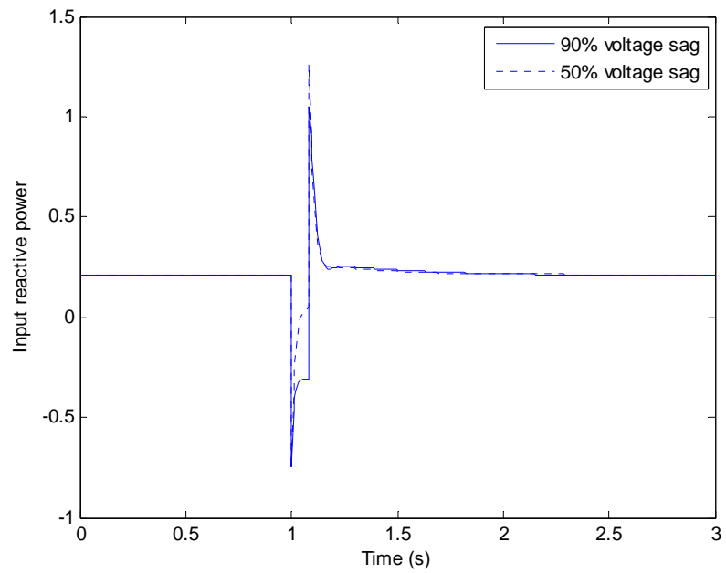
(c) The input reactive power (p.u.)
