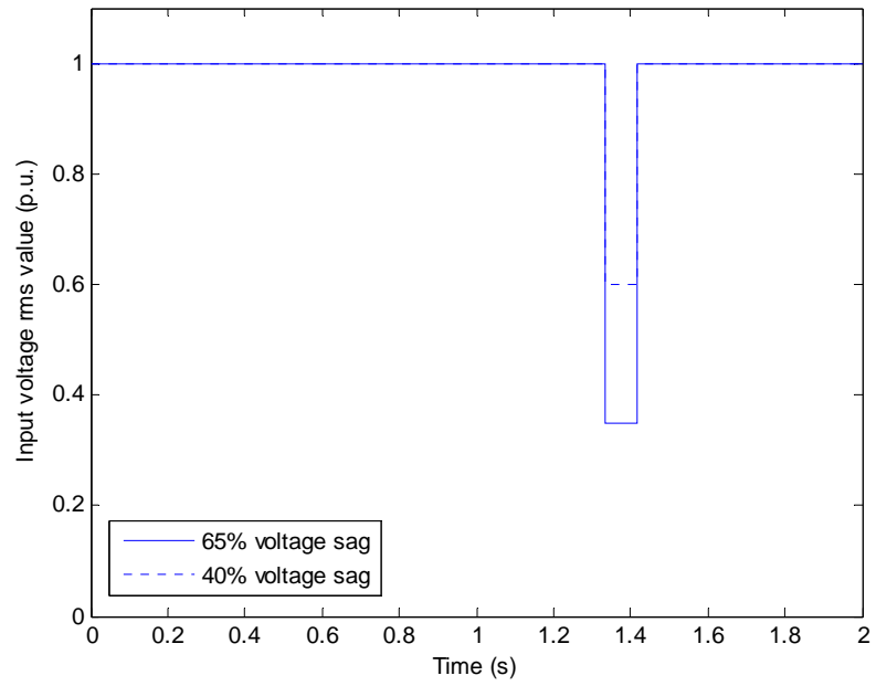
(a) The RMS value of the input voltage (p.u.)
