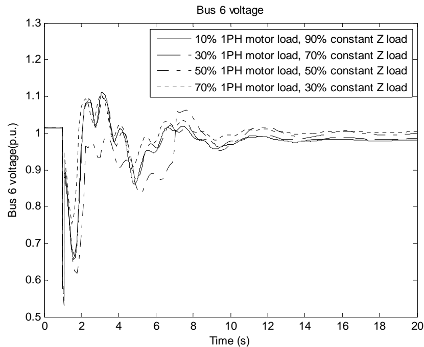
Figure 6-9 Bus 6 voltage magnitude with protection setup 2
