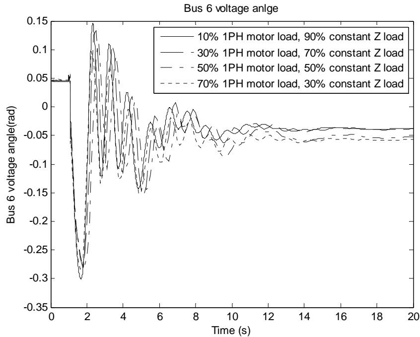
Figure 6-10 Bus 6 voltage angle with protection setup 2
