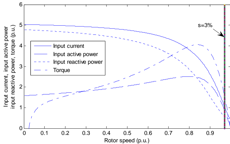
Figure 3-2 General characteristics of the three-phase induction motor
