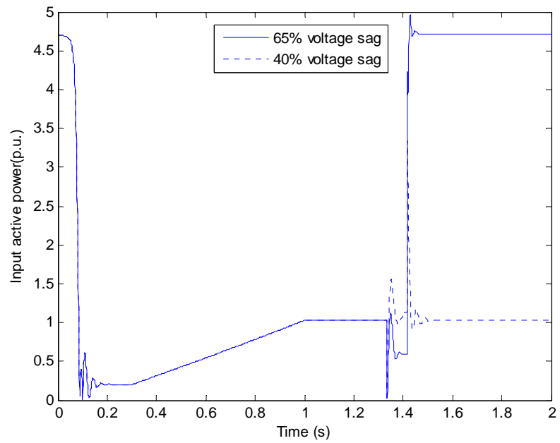
(b) The input active power (p.u.)
