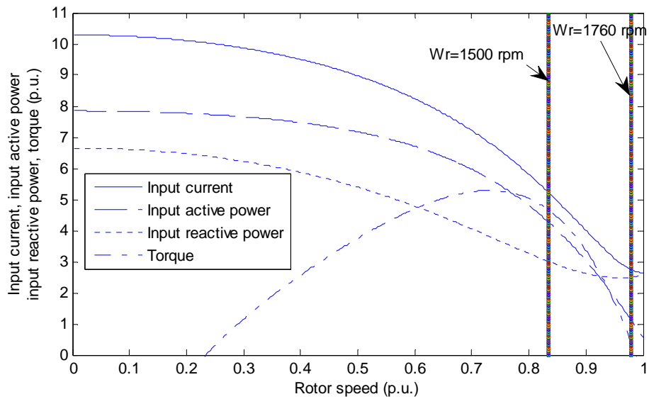
Figure 3-4 General characteristics of the single-phase induction motor
