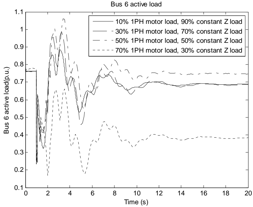
(a) Bus 6 load active power
