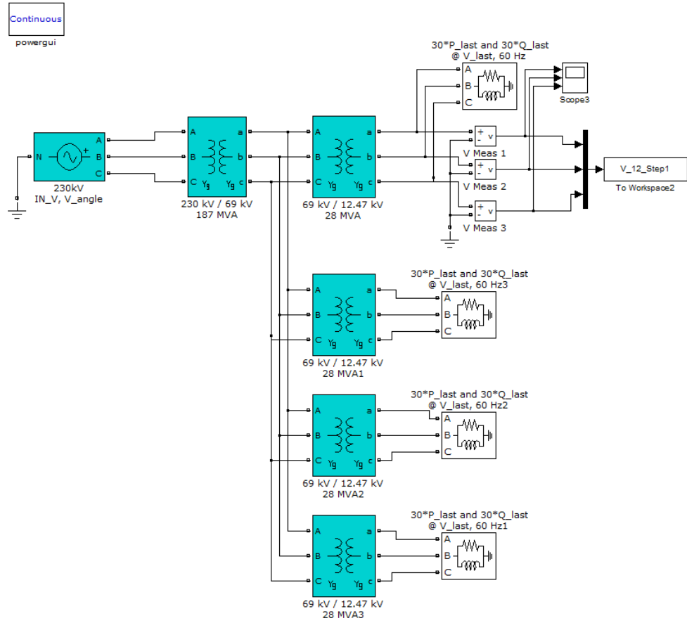
Figure A-1 Simulink step 1 for calculating end voltage after transformer
