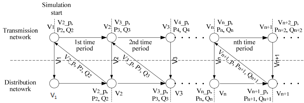
Figure 5-1 The simulation procedure of the power system
