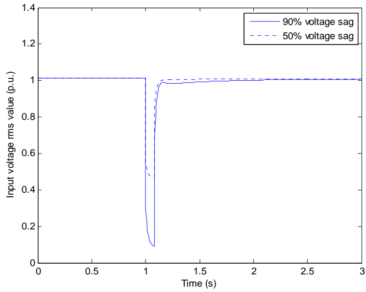
(a) The RMS value of the input voltage (p.u.)
