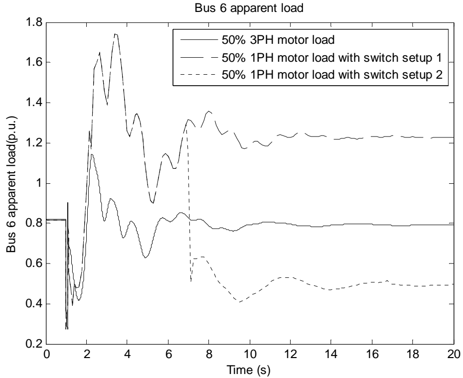
Figure 6-15 Bus 6 load for 50% motor load
