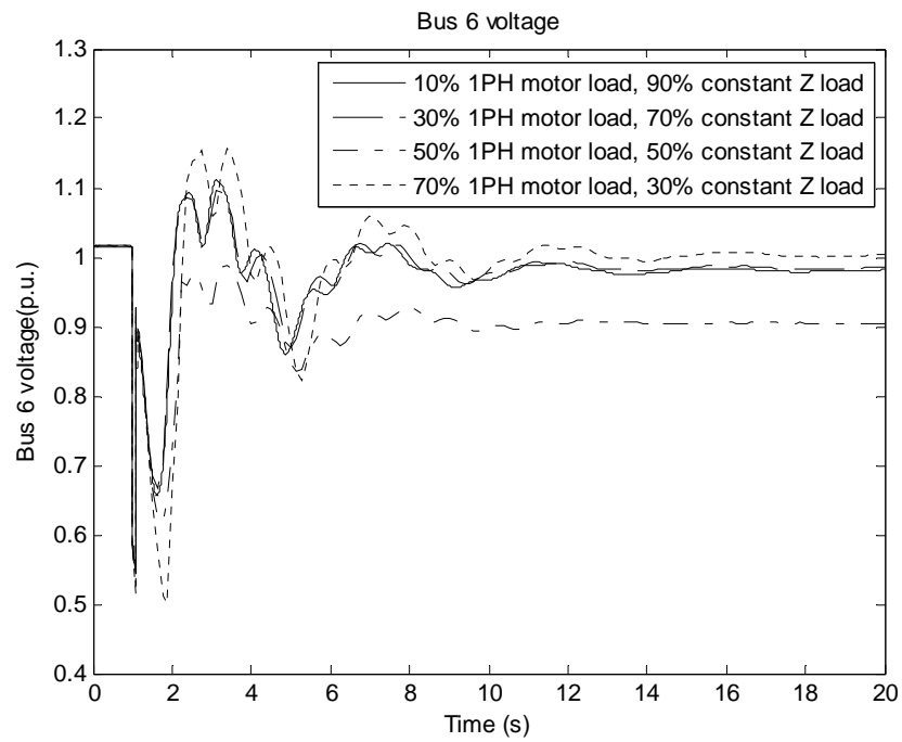
Figure 6-6 Bus 6 voltage magnitude with protection setup 1
