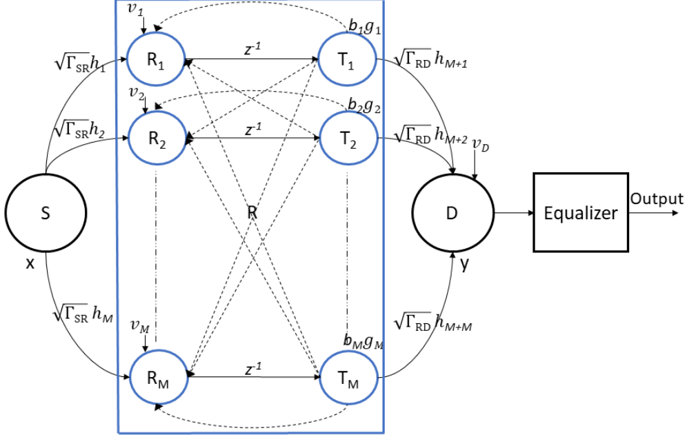
Figure 3.1: System model with source and destination nodes having one antenna without line of sight, connected by FD AF M \times M Relay
