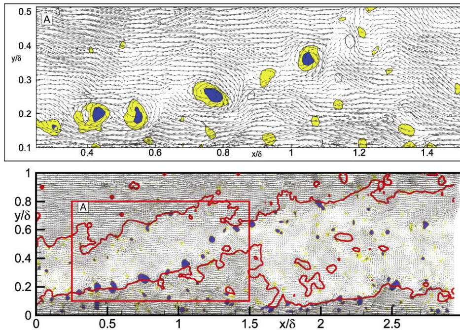
Figure 3 PIV measurements of the velocity field and vorticity field (colored contours) in a turbulent boundary layer flowing left to right. The ramp-like structures bounded by groups of concentrated vortices are evidence of hairpin vortex packets in which hairpins occur in a streamwise alignment with smaller, upstream hairpins auto-generated by larger, downstream hairpins. The velocity fields magnified in the upper inset figure possess the characteristics of hairpins identified in Figure 2 (from Adrian et al. 2000)..
