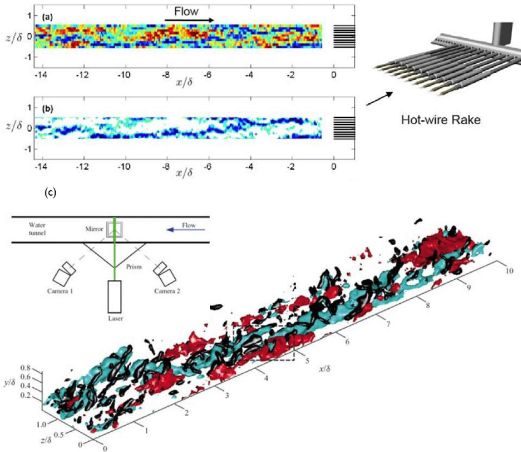
Figure 5 Very large-scale superstructure signatures: (a) From rake of hot wire traces from Hutchins and Marusic (2007); u signal at y/\delta = 0.15 for R_\tau = 14400 (b) Same with only low speed regions highlighted. (c). High-frame rate stereo-PIV measurements from Dennis and Nickels (2011a,b) in a turbulent boundary layer at R_\theta = 4700 , showing similar features to the hot-wire rake measurements. Here the black isocontours show swirl strength, indicating the corresponding location of vortical structures with the low-speed (blue) and high-speed (red) regions. After Marusic and Adrian (2013).
