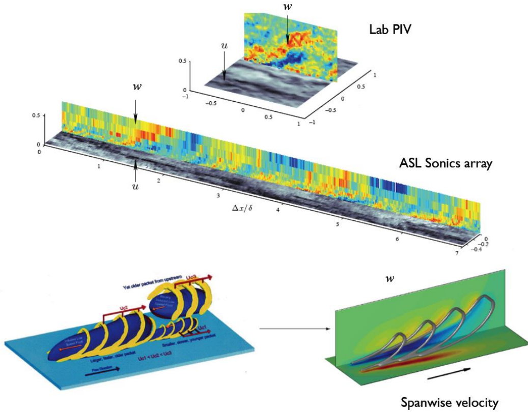
Figure 6 Top panel: Instantaneous velocity fluctuations in the streamwise-wall-normal ( x - y ) plane and instantaneous streamwise velocity fluctuations in the streamwise/spanwise ( x - y ) planes for data from laboratory PIV (Hambleton et al. 2006) and for the atmospheric surface layer using an arrays of sonic anemometers (Hutchins et al. 2012). High positive w regions are indicated by red while blue denotes highly negative w regions. High negative u regions are indicated by dark gray while light gray shade denotes highly positive u regions. Bottom panel shows the Biot Savart law calculations for an idealized packet of hairpin vortices with their image vortices in the wall, as per the schematic of Adrian et al. (2000) shown on the left side.
