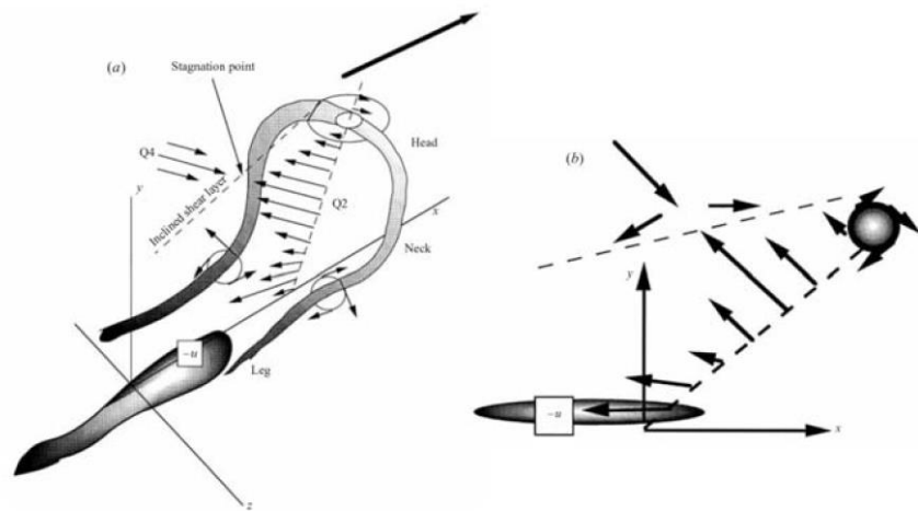
Figure 2 Schematic of hairpin eddy attached to the wall; (b) signature of the hairpin eddy in the streamwise/wall-normal plane (from Adrian et al. 2000).
