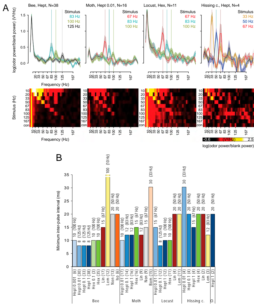
Fig. 3. Antennal responses track pulses at 125 Hz in a 1-s-long odor stimulus. ( A ) Periodograms (mean \pm SEM) of the EAG responses for the three highest resolved pulse frequencies for different insects in different insect species, and color-coded periodograms for all pulse series for the same species-odor combination. A peak in the periodogram indicates that the EAG response followed that stimulus frequency. ( B ) Temporal resolution of EAG responses quantified as the minimum inter-pulse interval in milliseconds ( 1/\text{maximum pulse frequency} ) that an EAG response could follow. Minimum inter-pulse intervals were determined by locating the peak of the average periodogram in a \pm 20 -Hz window around the stimulus frequency. Pulse following was ascertained if the negative SE of the peak location rose above the positive SE of the trough location within that window. The corresponding pulse tracking frequencies are given in parentheses above the odorant.
