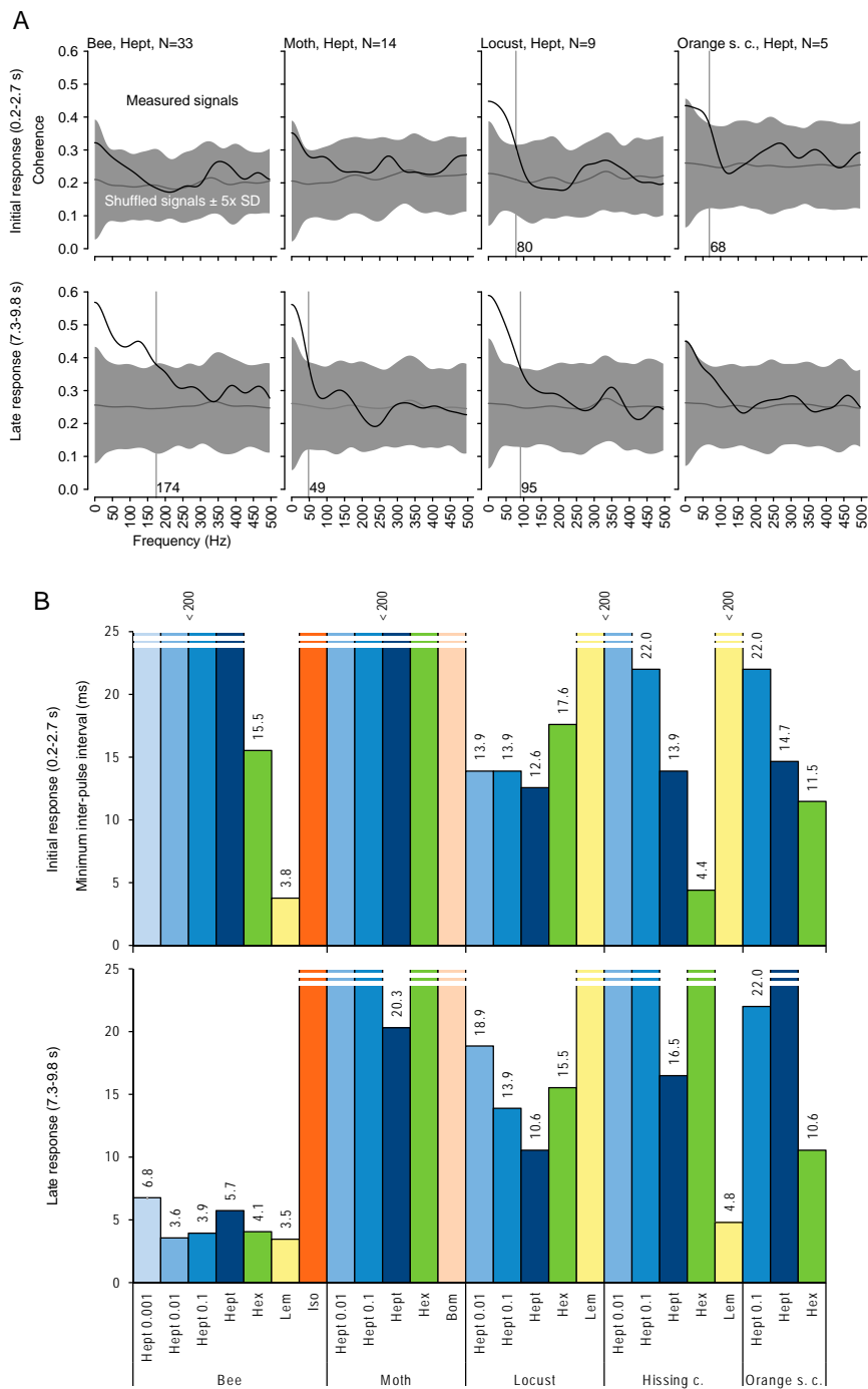
Fig. 5A. Temporal resolution of EAG responses during initial and late odor responses. (A) Coherence between c. EAG responses and smoke signals measured during the initial (0.2–2.7 s) and late (7.3–9.8 s) period of a 10-s-long broadband frequency stimulus train with random pulse durations. The values at the vertical lines show the maximum EAG frequency responses with significant coherence. (B) Temporal resolution of EAG responses quantified as the minimum inter-pulse interval (1/maximum pulse frequency) at which the coherence is still significant.
