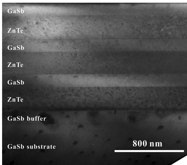
FIG. 3. Low-magnification TEM image of a ZnTe/GaSb DBR sample with seven \lambda/4 pairs.
