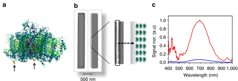
Figure 2 | Coupling of PS I to a free-standing Au microcavity. (a) PS I structure. The cysteine mutations used to bind the PS I to the metal surface are depicted in yellow space-filled sulfur atoms and indicated by arrows. (b) Left: SEM images of an uncoated 440 \times 4,500 nm single slit (left) and a slit that is adsorbed with three PS I layers (right). Right: zoom of the coated slit corresponds to layer thickness of 33 \pm 4 nm (three layers) that is formed on the walls of the slit, leaving the majority of the slit vacant. (c) Normalized transmission of light through 440 \times 4,500 nm single slit adsorbed with a multilayer composed of three PS I layers (red), in comparison with transmission through an uncoated slit (blue). Transmission of light (far-field) through the coated slit is enhanced by a factor of 13 in comparison with the slit not coated with molecules.
