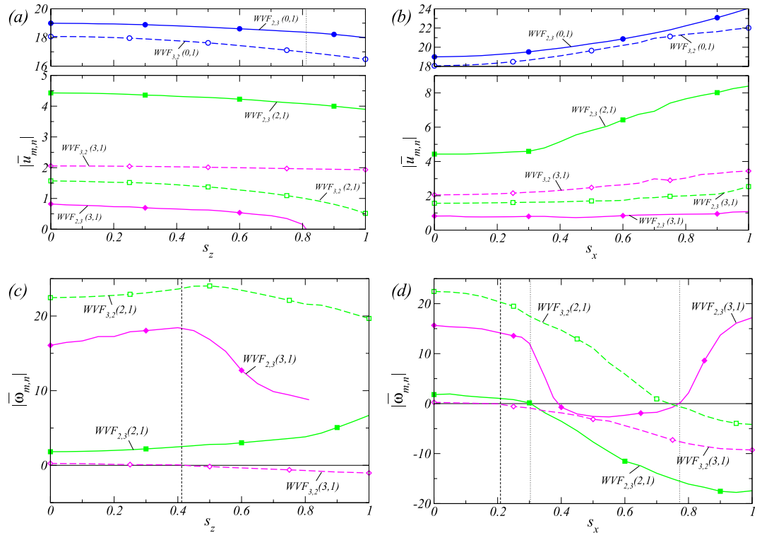
Figure 4. Bifurcation with the strength of magnetic field. Variation of WVF_{2,3} ( WVF_2 ) and WVF_{3,2} with axial (left column) and transverse (right column) magnetic field strength. Shown are (a,b) time-averaged, dominant amplitudes |\bar{u}_{m,n}| of the radial velocity field at mid-gap contributed from the axisymmetric mode [(m, n)=(0,1)] , the m = 2 mode [(m, n) = (2,1)] , and the m = 3 mode [(m, n) = (3,1)] , respectively. (c,d) The corresponding time-averaged frequency |\bar{\omega}_{m,n}| of the complex mode amplitudes u_{m,n}(r, t) . Symbols are for eye guidance (the same for subsequent figures), but calculations were typically done for many more parameter values. All presented solutions are stable. The vertical dashed (dotted) lines indicate the critical magnetic field strength in s_x ( s_z ) at which the WVF_{3,2} ( WVF_{3,2} ) flow changes its direction of rotation (cf. Fig. 3): \omega_{3,1}(WVF_{3,2}) = 0 for s_z = 0.427 , \omega_{3,1}(WVF_{2,3}) = 0 for s_x = 0.209 , \omega_{2,1}(WVF_{2,3}) = 0 for s_x = 0.309 , and \omega_{2,1}(WVF_{2,3}) = 0 for s_x = 0.772 . Note that the events \omega_{2,1}(WVF_{3,2}) = 0 at s_x = 0.738 and \omega_{3,1}(WVF_{2,3}) = 0 at s_z = 0.378 do not reverse the rotational direction of the respective wavy flows (See, Figure 3).
