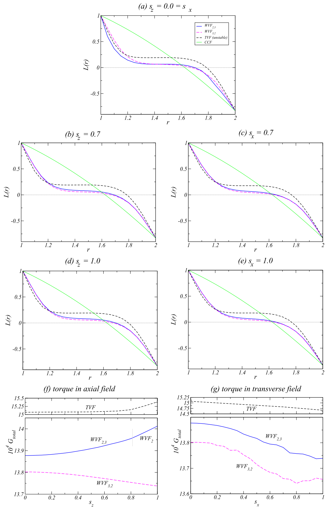
Figure 9. Angular momentum and torque. (a–e) Angular momentum L(r) = r \langle v(r) \rangle_{0,z} / Re_1 scaled with the inner Reynolds number versus the radius r for the solutions: WVF_{2,3} ( WVF_2 for s_z = 1.0 ), WVF_{3,2} , unstable TVF, and CCF for s_x and s_z values as indicated. (f,g) Variation with s_z and s_x of the dimensionless torque G = \nu \omega (see text for details) for WVF_{2,3} ( WVF_2 ) and WVF_{3,2} .
