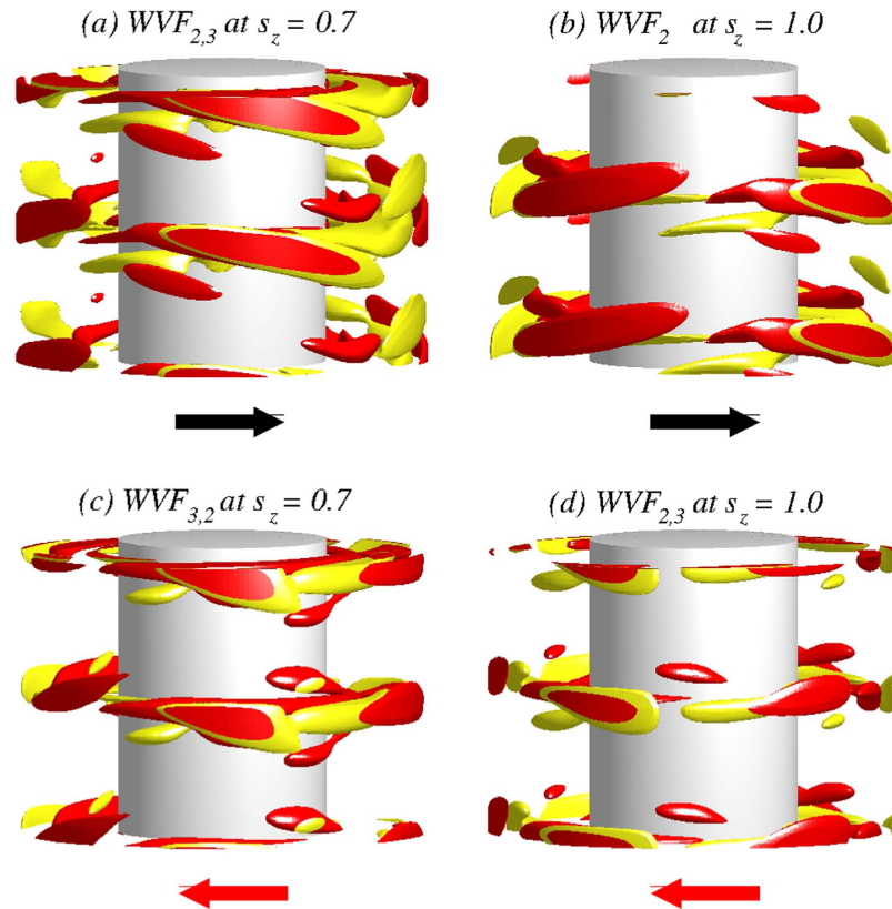
Figure 5. Structural properties of flows in the presence of an axial magnetic field. Isosurfaces of \eta for WVF_{2,3} , WVF_{3,2} and WVF_2 for s_z = 0.7 and s_z = 1.0 . Vorticity isosurfaces are for \eta = \pm 240 , and two periods of motion are plotted in the axial direction. The arrows below the snapshots illustrate the rotational direction, which appears laterally on the cylinders. For these values of s_z the flow pattern of WVF_{2,3} is pro-grade but that of WVF_{3,2} is retrograde. See also movie files movie3.avi and movie4.avi in SMs.
