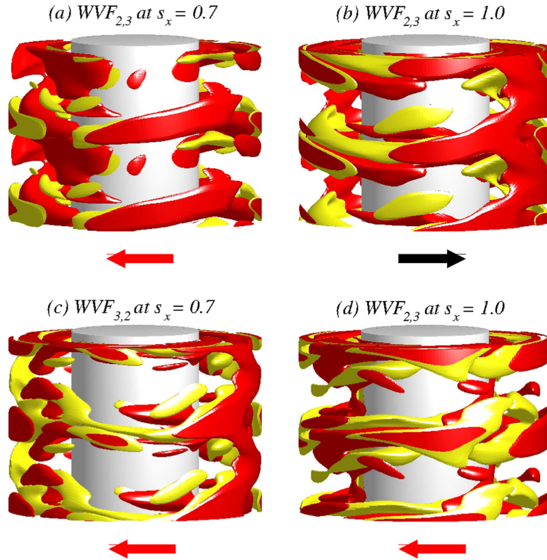
Figure 7. Flow structures in a transverse magnetic field. Isosurfaces of \eta for WVF_{2,3} and WVF_{3,2} for transverse magnetic field strength s_x = 0.7 and s_x = 1.0 . Vorticity isosurfaces are \eta = \pm 240 and two periods are plotted in the axial direction. The arrows below the snapshots illustrate the rotational direction (appearing laterally on the cylinders). For s_x = 0.7 , the WVF_{2,3} flow is pro-grade but for s_x = 1.0 , it is retrograded. The WVF_{3,2} flow is retrograde for both values of s_x (cf. Fig. 5). See also movie files movie5.avi, movie6.avi and movie7.avi in SMs.
