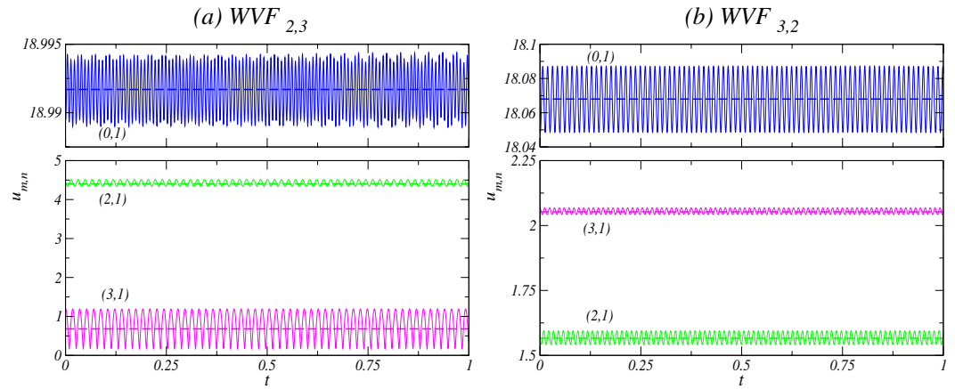
Figure 2. Time evolution of dominant flow amplitudes. Flow states of WVF_{2,3} (left panels) and WVF_{3,2} (right panels) for s_z = 0 and s_x = 0 . Shown are time-dependent [and time-averaged (dashed lines)], dominant amplitudes u_{m,n} [ \bar{u}_{m,n} ] of the radial velocity field at mid-gap contributed by the axisymmetric mode [( m, n ) = (0,1)], the m = 2 mode [( m, n ) = (2,1)], and the m = 3 mode [( m, n ) = (3,1)], respectively.
