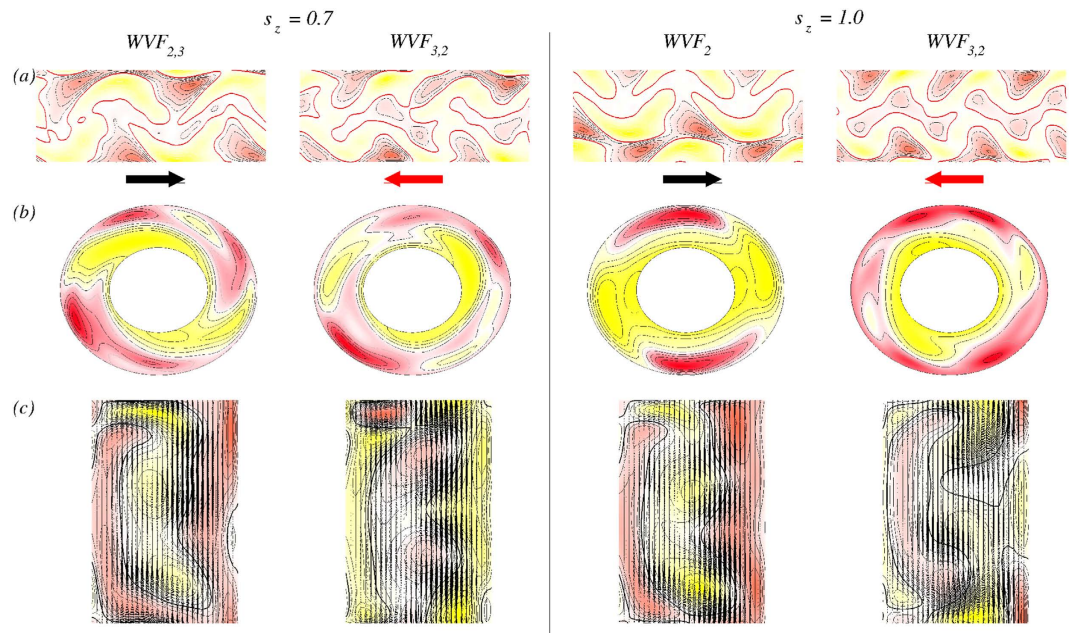
Figure 6. Flows in the presence of an axial magnetic field (cf. Fig. 5). Contours of flows for s_z values as indicated. (a) Contour of the radial velocity u(\theta, z) on an unrolled cylindrical surface in the annulus at mid-gap. The arrows below illustrate the rotational direction. (b) Contour of the velocity component u in the (r, \theta) plane at mid-height. (c) Vector plots [u(r, z), w(r, z)] of the radial and axial velocity components in a constant \theta plane, with color-coded azimuthal vorticity \eta from red (minimum) to yellow (maximum). See also movie files movie3.avi and movie4.avi in SMs.
