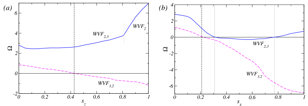
Figure 3. Pro-grade and retrograde wavy flows in presence of a magnetic field. Variations in the angular velocity \Omega of the wavy states in the presence of axial [ s_z \neq 0 but s_x = 0 , (a)] and transverse [ s_x \neq 0 but s_z = 0 , (b)] magnetic field. Vertical dotted and dashed lines indicate the points of non-rotating flow pattern, i.e., standing waves, which are the reversal points of the motion for WVF_{2,3} and WVF_{3,2} , respectively. The horizontal black line indicates zero angular velocity. For axial field strength s_z \gtrsim 0.812 , there is wavy flow WVF_2 without any m = 3 contribution, where the short thin gray line marks the bifurcation point. With axial field only WVF_{3,2} changes its propagating direction for s_z \approx 0.427 . With transverse field both wavy flows change their propagation directions: WVF_{3,2} at s_x \approx 0.209 and WVF_{2,3} twice, first for s_x \approx 0.309 to retrograde and second for s_x \approx 0.772 back to prograde behavior. For WVF_{2,3} the minimal angular velocity \Omega_{\min} = -0.325 is achieved for s_x \approx 0.58 .
