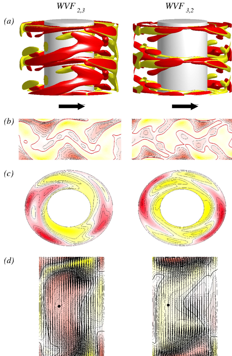
Figure 1. Flow structures in absence of any magnetic field. Flow states of WVF_{2,3} (left panels) and WVF_{3,2} (right panels) for s_z = 0 and s_x = 0 . (a) Isosurfaces of \eta = \pm 240 . Red (yellow) color indicates positive (negative) vorticity. For clear visualization, two periods are plotted in the axial direction. The arrows below the snapshots illustrate the rotational direction (appearing laterally on the cylinders), which is pro-grade for both wavy flows. Note, here and in the following the rotation direction always refers to the pattern rotation. Contours of the flow structures: (b) radial velocity u(\theta, z) on an unrolled cylindrical surface in the annulus at mid-gap, (c) azimuthal vorticity \eta in the (r, \theta) plane at mid-height, and (d) vector plots (u(r, z), w(r, z)) of the radial and axial velocity components in a constant \theta = plane, including the azimuthal vorticity \eta . The two points mark the centerline of vortices within the illustrated plane. Note that this position is \theta -dependent but the azimuthal averaged position for WVF_{3,2} is closer to the inner cylinder than for WVF_{2,3} . All contours are color coded from red (dark gray - minimum) to yellow (light gray - maximum). See also movie files movie1.avi and movie2.avi in SMs.
