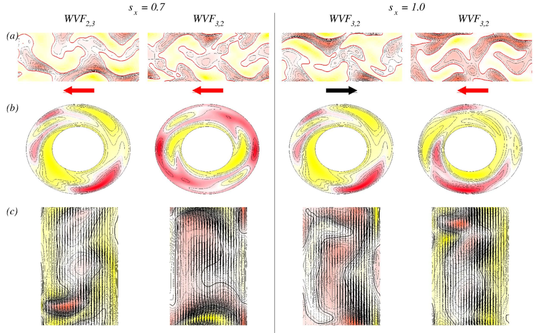
Figure 8. Flow structures in a transverse magnetic field (cf. Fig. 7). (a) Contours of the radial velocity u(\theta, z) on an unrolled cylindrical surface in the annulus at mid-gap. The arrows below illustrate the rotational direction. (b) Contours of the velocity component u in the (r, \theta) plane at mid-height. (c) Vector plots [u(r, z), w(r, z)] of the radial and axial velocity component in a constant \theta = \text{plane} , with color coded azimuthal vorticity \eta from red (minimum) to yellow (maximum). See also movie files movie5.avi, movie6.avi and movie7.avi in SMs.
