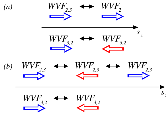
Figure 10. Summary: schematic illustration of flow reversal with magnetic field strength: (a) axial field and (b) transverse field. Thick arrows below the terms indicate the rotating directions of the corresponding flow patterns, which appear lateral on the cylinder. Note that the sequences hold for increase and decrease of magnetic field strength.
