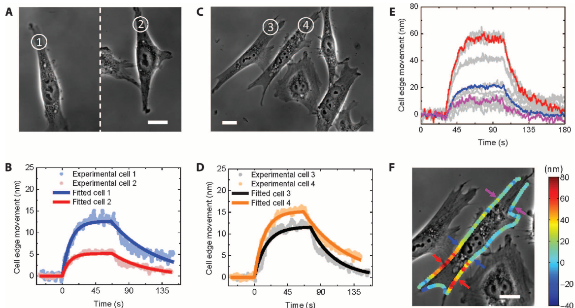
Fig. 4. Heterogeneity of small-molecule interactions with cell membrane receptors. (A and C) Phase-contrast images of fixed \alpha 4\beta 2 -transfected SH-EP1 cells, where the numbers mark the cells under analysis. Scale bars, 20 \mu\text{m} . (B) Binding kinetics of cells 1 and 2 (100 nM acetylcholine). (D) Binding kinetics of cells 3 and 4 (100 nM acetylcholine). (E) Binding kinetics at different locations of the cell in (F) (100 nM acetylcholine). (F) Phase-contrast image of a fixed \alpha 4\beta 2 -transfected SH-EP1 cell. The color represents the amount of cell membrane edge deformation. Scale bar, 20 \mu\text{m} .
