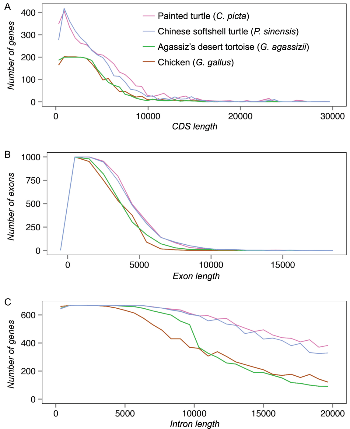
Fig 3. Gene structure of Gopherus agassizii compared to other reptiles. Frequency distribution of genes or exons relative to (A) coding DNA sequence (CDS) lengths, (B) exon length and (C) intron length of Agassiz's desert tortoise, chicken [74], western painted turtle [18], and Chinese softshell turtle [17]. CDS is for genes less than 10 kb.
