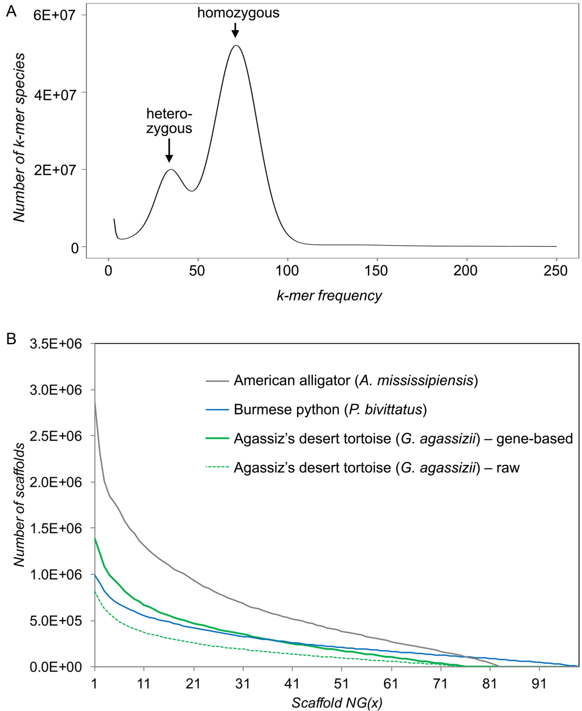
Fig 1. Assembly statistics for the genome of Gopherus agassizii and comparison with Python bivittatus and Alligator mississippiensis . (A) Two k-mer frequency peaks exist for G. agassizii : a peak at 35X coverage, representing heterozygous regions and a peak at 71X coverage, representing homozygous regions. (B) Gene-based scaffolding greatly increased scaffold N50 from 169.2 kbp to 251.6 kbp, which places it within the range of recently published genomes of reptiles including the Burmese python [71] and the American alligator [72].
