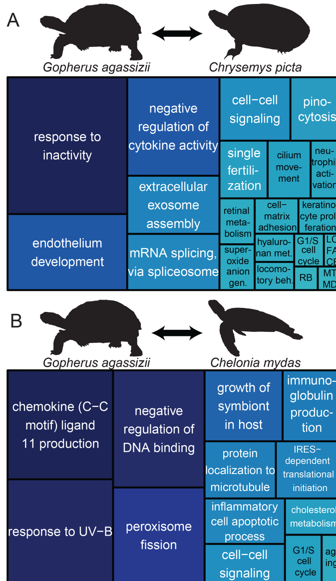
Fig 5. Comparative genomics of chelonians. Representation of Gene Ontology terms for biological processes shared by genes with pairwise Ka/Ks > 1 in comparisons of Gopherus agassizii to (A) Chrysemys picta bellii and (B) Chelonia mydas . Treemap boxes are both sized and colored by uniqueness. Abbreviations in (A): RB, receptor biosynthesis, LCFACB, long chain fatty acyl-CoA biosynthesis, MTMD, membrane to membrane docking.
