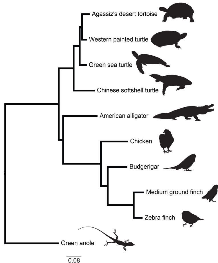
Fig 4. Phylogeny of 10 sauropsids including Gopherus agassizii . Phylogeny shows the relationships of sauropsids, including four chelonians, with complete genome sequences. Branch lengths are given in terms of DNA substitutions per site derived from fourfold degenerate sites.
