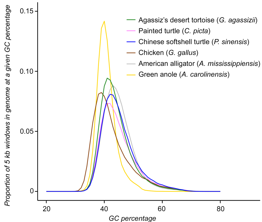
Fig 2. Frequency distribution (proportion) of GC content calculated in 5 kbp non-overlapping windows for Gopherus agassizii and other reptilian genomes. GC content of G. agassizii closely matches that of the turtles Chrysemys picta bellii and Pelodiscus sinensis [17,18], and overlaps the American alligator ( Alligator mississippiensis ) [72], the green anole ( Anolis carolinensis ) [73], and the chicken ( Gallus gallus ) [70].
