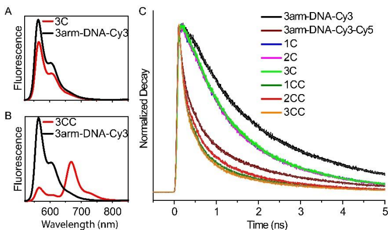
Figure 4. Fluorescence emission spectra of 3C (A) and 3CC (B) in comparison with emission spectra of 3arm-DNA-Cy3 ( \lambda_{\text{ex}} = 510 nm). (C) Cy3 fluorescence decay profiles of free 3arm-DNA and 3arm-DNA conjugated to the RC in various ratios, with either constructs containing Cy3 alone ( 1C , 2C , 3C ) or constructs with both Cy3 and Cy5 ( 1CC , 2CC , 3CC ), monitored at 565 nm ( \lambda_{\text{ex}} = 510 nm).
