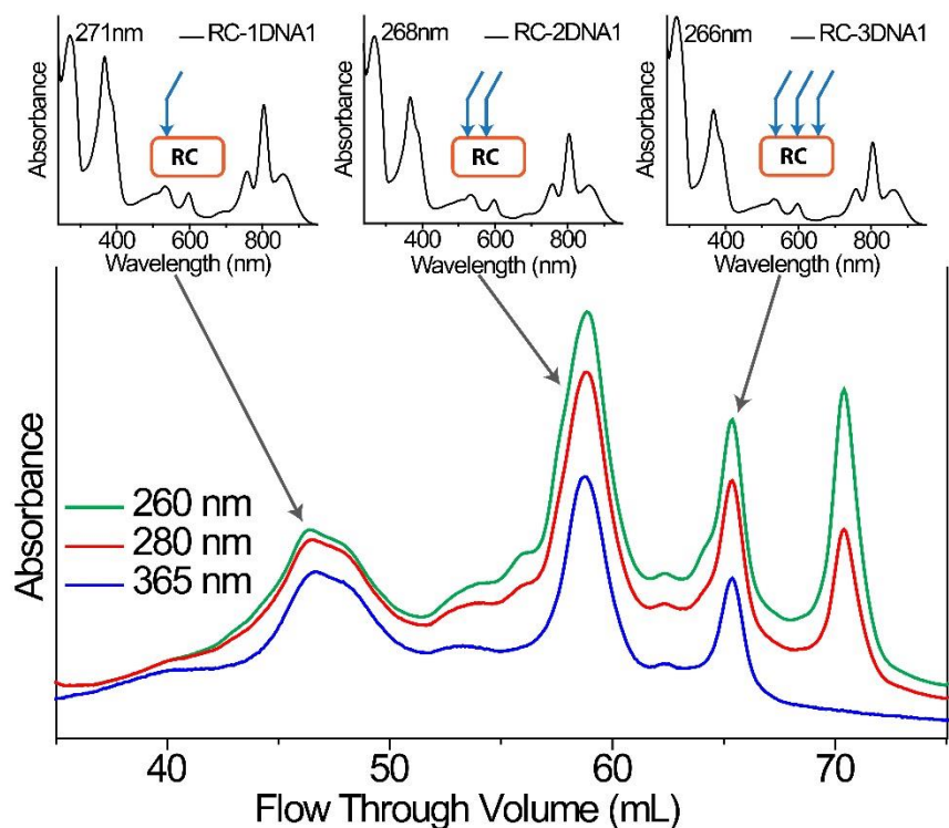
Figure 2. FPLC purification trace of DNA (Strand-1) conjugated RCs. Chromatographs at 260 nm (green), 280 nm (red) and 365 nm (blue) are shown. The absorbance bands at 260 nm and
