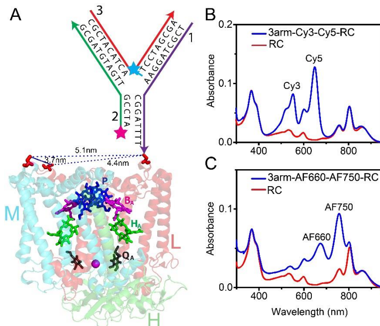
Figure 1. (A) Modified structure of the reaction center (RC) from the purple bacterium, Rhodospirillum rubrum 2.4.1 (PDB 2J8C) with sequences of the 3arm-DNA construct shown. The cofactors of the RC are colored and those active in electron transfer reactions involved in this report are designated by letters: P – bacteriochlorophyll pair, B A – bacteriochlorophyll monomer, H A – bacteriopheophytin, Q A – ubiquinone. The arrows in the DNA structure point in direction of the 3' end of the DNA strands. The 3'-Amine modified Strand-1 (purple) of the 3arm-DNA is conjugated to one of the Cys residues (shown in red) on the surface of the RC via a SPDP (N-succinimidyl 3-(2-pyridyldithio) propionate) linker. The other two strands (Strand-2 and -3 in green and red, respectively) are allowed to hybridize to Strand-1 to form the 3arm-DNA junction. Inter-Cys distances on the RC are marked as dotted lines. The two stars on 3arm represent the positions of the two dye molecules, where the cyan star corresponds to either Cy3 or AF660, and the pink star corresponds to either Cy5 or AF750. It should be noted that because of the presence of three Cys residues on the surface of the protein, 1 or 2 or 3 copies of Strand-1 can be conjugated to the RC, and consequently up to three 3arm-DNA junctions (and three pairs
