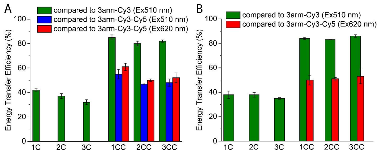
Figure 5. Energy transfer efficiency of 3arm-DNA conjugated RC calculated from (A) steady-state data and (B) from lifetime data. The green bars show energy transfer efficiency calculated by comparing fluorescence from the RC containing complex with that from the 3arm-DNA containing only Cy3 (without RC). The blue and red bars are the energy transfer efficiency values calculated with excitation of Cy3 and Cy5 respectively, using the 3arm-DNA containing both the dyes (Cy3-Cy5) without the RC attached as the fluorescence reference. The FRET efficiencies (E) from steady-state fluorescence data were calculated according to the following
