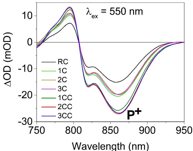
Figure 6. Light-minus-dark difference absorbance spectra of RCs with and without conjugation to a 3arm-DNA nanostructure-dye complex.
