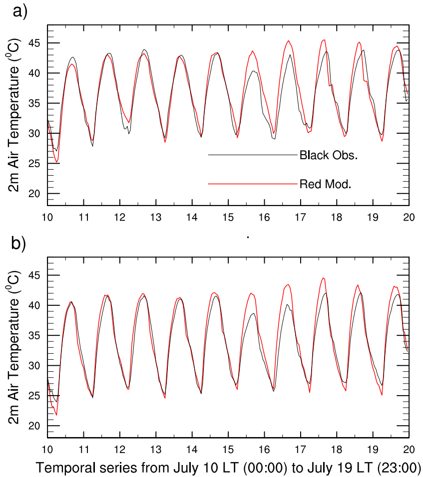
Figure 3. (a) Time series of the observed (black line) and modeled (red line) 2-m air temperature ( ^{\circ}\text{C} ) for the urban stations during the 10-day EWD period in July 2009. (b) As in (a) but for the rural stations.
