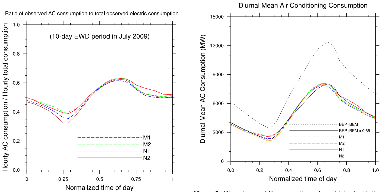
Figure 4. Ratio of AC consumption to total electric consumption averaged for the 10-day EWD period in July 2009 computed with the four methodologies: M1, M2, N1, and N2.
